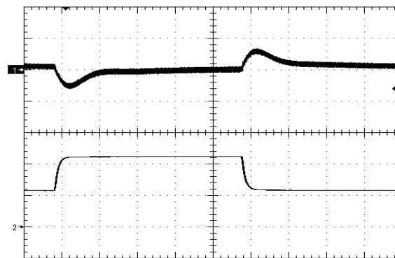
Figure 12. Load Transient Response (50mV/div), di/dt=0.1A/uS, 25% - 50% - 25% of full load, +2000uF Oscon, time scale: 200uS/div
