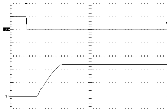
Figure 10. Startup Waveform via Enable Pin, time scale 10mS/div. Vin=Vin_nom, full resistive load + 2200uF (negative enable.) Ch1,Ch2=5V/div
