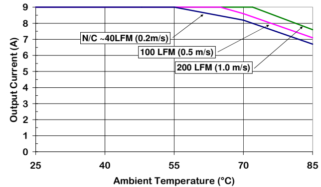
Figure 6. Output Current Derating vs Ambient Temperature & Airflow (air flowing from pin 3 to pin 1, Vin = 24 V, with baseplate)
