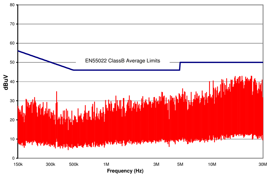
Figure 18. CPE9B36 Conducted Emissions using above specified input filter, Vin = 48V, Full Resistive Load
