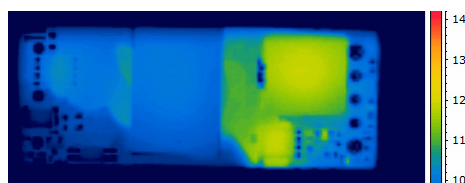
Thermal Image of module @ 48Vin, 200LFM & 55C
