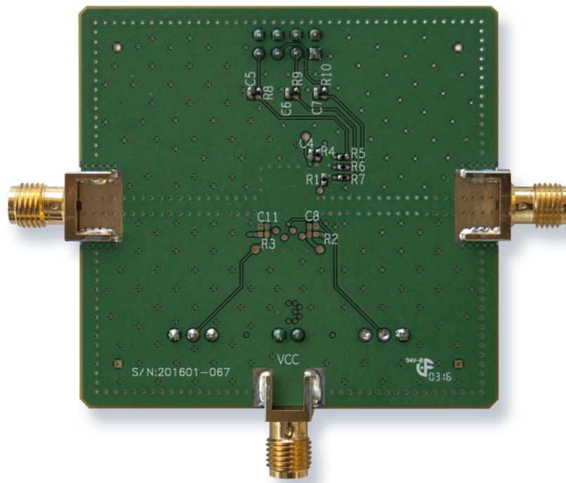
Figure 66. Bottom View
