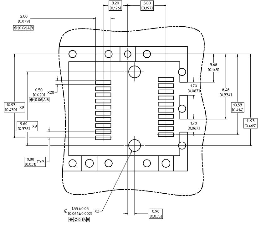
DETAIL 1 SCALE 10:1
