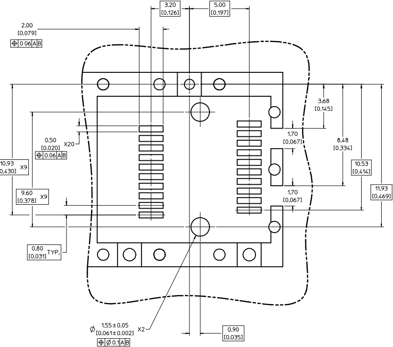
DETAIL 1 SCALE 10:1
