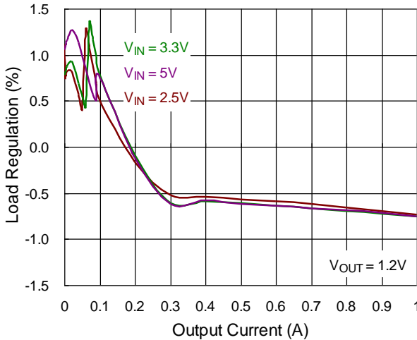
Load Regulation
