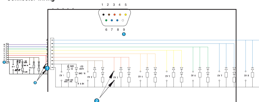
Connector wiring
