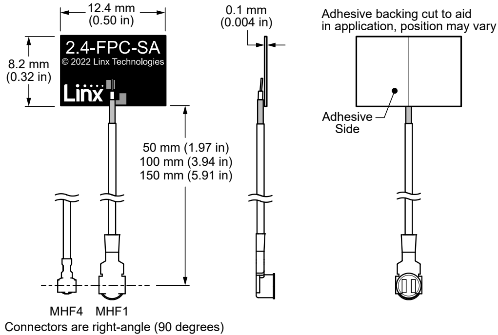
Figure 1. ANT-2.4-FPC-SAH Series Antenna Dimensions
