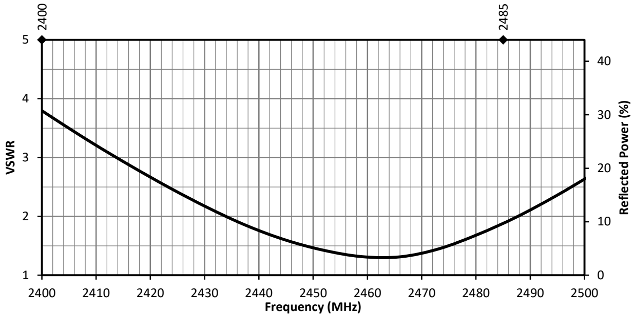
Figure 2. ANT-2.4-FPC-SAH Antenna VSWR
