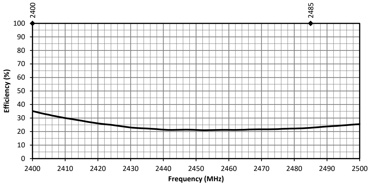
Figure 6. ANT-2.4-FPC-SAH Antenna Radiation Efficiency
