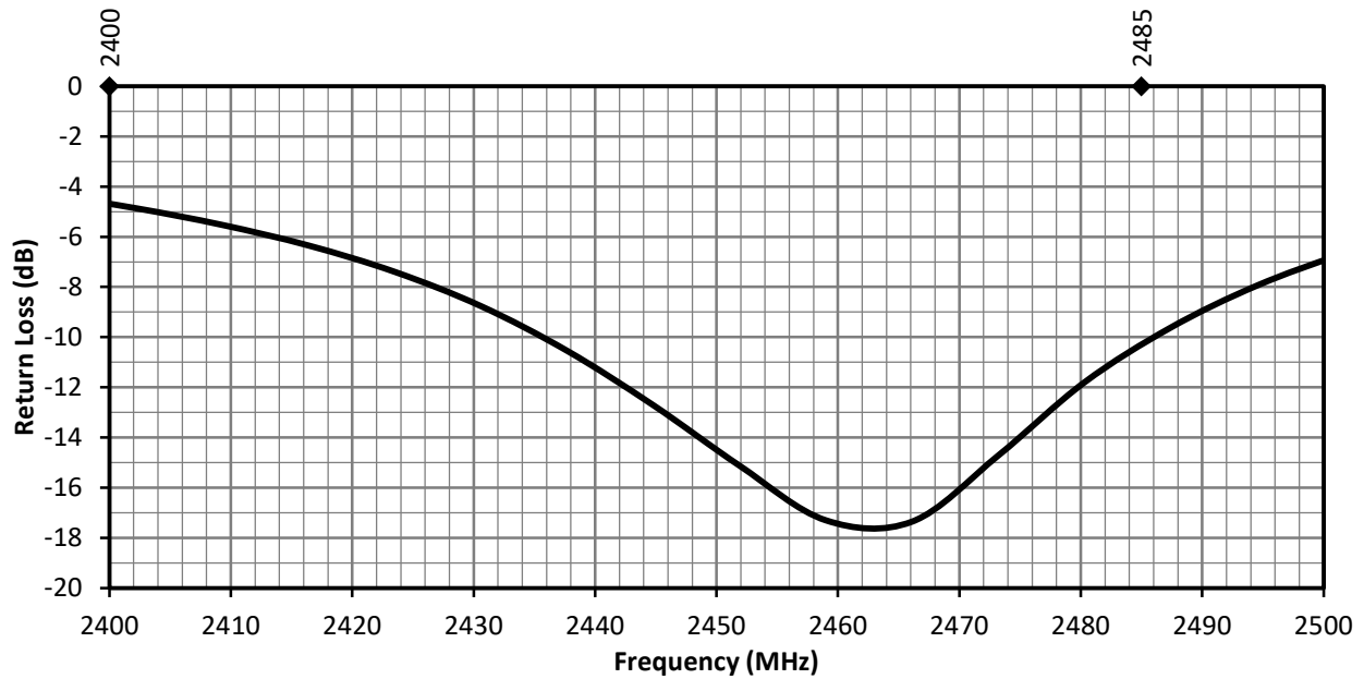
Figure 3. ANT-2.4-FPC-SAH Antenna Return Loss
