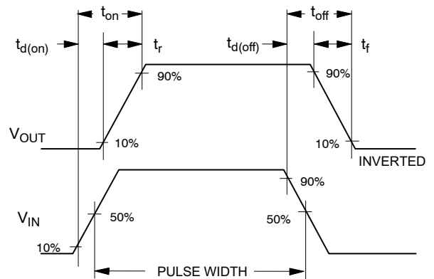
Figure 12. Switching Waveforms
