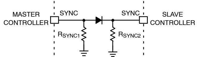
Figure 50. Master-Slave Configuration
