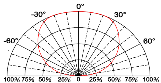
Fig.6 Directive Radiation
