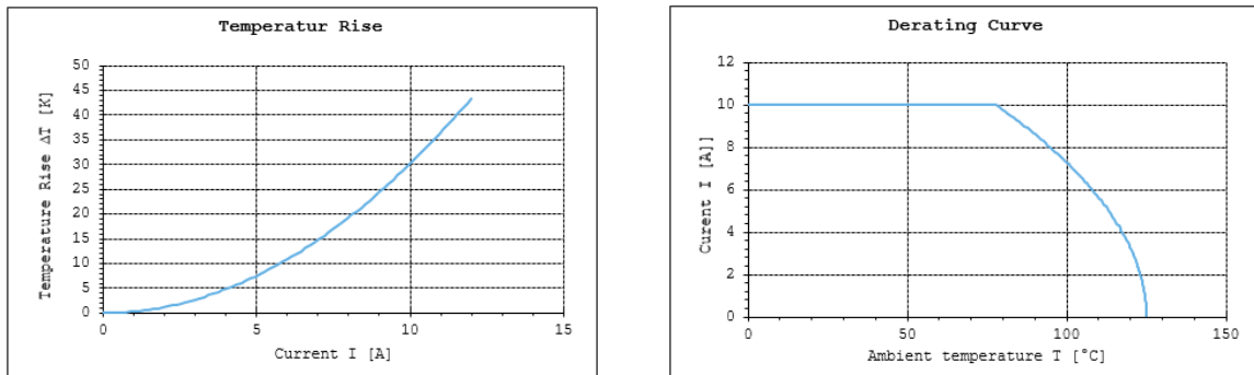
Figure 4. Current &amp; Temperature-rise Curve, and Derating Curve of TE UPM STD 12P power
