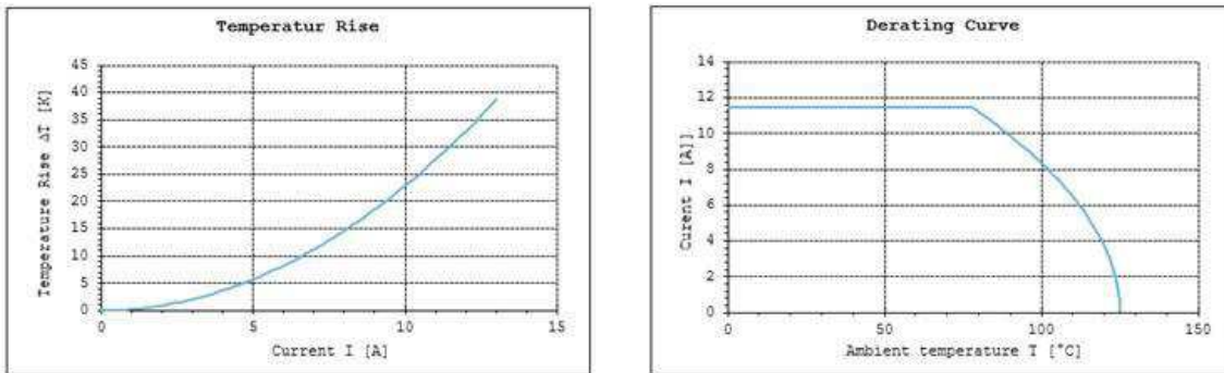
Figure 2. Current &amp; Temperature-rise Curve, and Derating Curve of TE UPM STD 4P power
