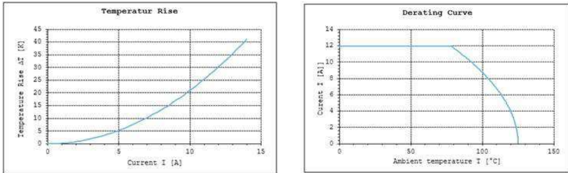
Figure 1. Current &amp; Temperature-rise Curve, and Derating Curve of TE UPM STD 3P power
