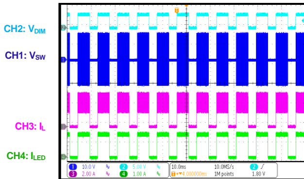
PWM Dimming Steady State Dimming frequency = 120Hz/5ms
