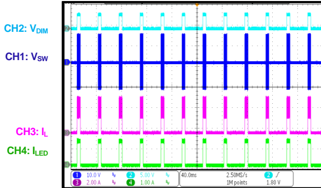
PWM Dimming Steady State Dimming frequency = 30Hz/5ms
