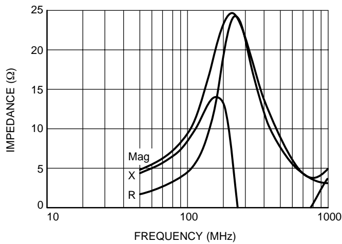
Figure 5. Typical Impedance vs. Frequency
