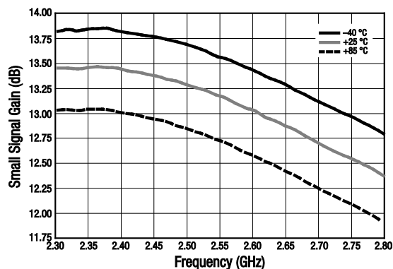
Figure 5. Small Signal Gain (Narrow Band) vs Frequency Over Temperature
