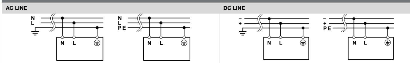
FIG.7 - INPUT CONNECTIONS
