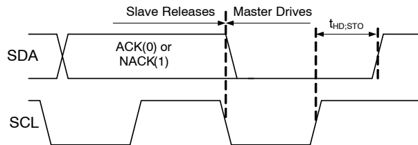
Figure 39. Stop Bit
