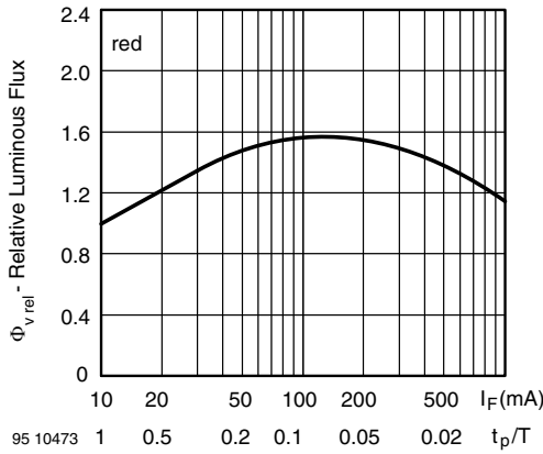
Fig. 7 - Relative Luminous Flux vs. Forward Current/Duty Cycle
