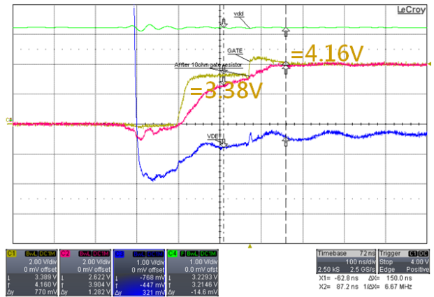
Figure 15. V_{OH} Level with C_{CP} = 2.2\text{ nF} (ch1: GATE pin; ch2: MOSFET Vgs; ch3 : VRAIN : ch4 : VDD)
