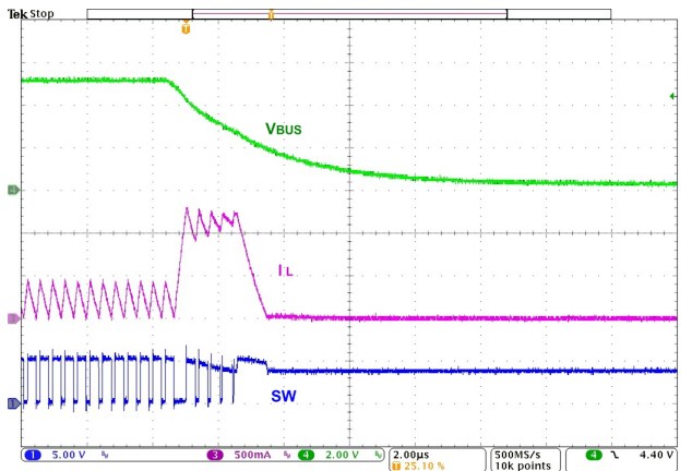
Figure 31. V_{BUS} Fault Response, 3.6\text{ V}_{BAT}
