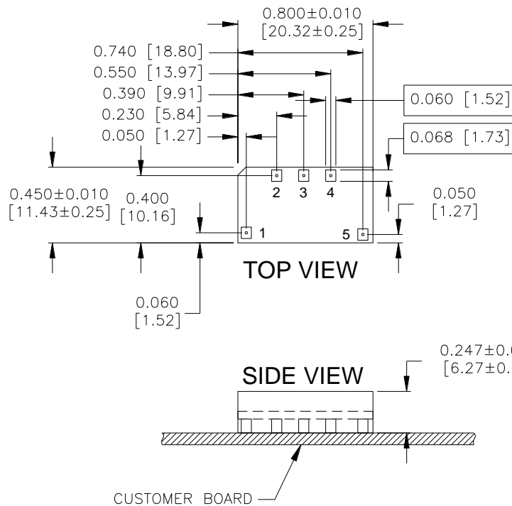
YM12S Pinout (Surface Mount)
