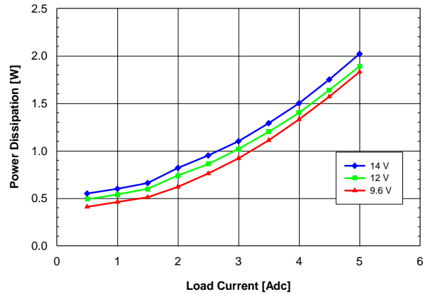
Fig. 2.5V.4: Power Loss vs. load current and input voltage for V_{out} = 2.5V converter mounted vertically with air flowing from pin 5 to pin 1 at a rate of 200 LFM (1 m/s) and T_a = 25^\circ C .
