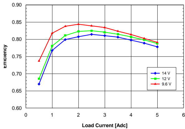
Fig. 1.2V.3: Efficiency vs. load current and input voltage for V_{out} = 1.2V converter mounted vertically with air flowing from pin 5 to pin 1 at a rate of 200 LFM (1 m/s) and T_a = 25\text{ }^{\circ}C .
