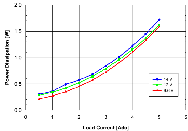
Fig. 1.2V.4: Power Loss vs. load current and input voltage for V_{out} = 1.2V converter mounted vertically with air flowing from pin 5 to pin 1 at a rate of 200 LFM (1 m/s) and T_a = 25\text{ }^{\circ}C .
