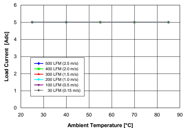
Fig. 1.5V.2: Available load current vs. ambient temperature and airflow rates for V_{out} = 1.5V converter mounted horizontally with V_{in} = 12V , air flowing from pin 5 to pin 1 and maximum MOSFET temperature \leq 120^\circ C .
