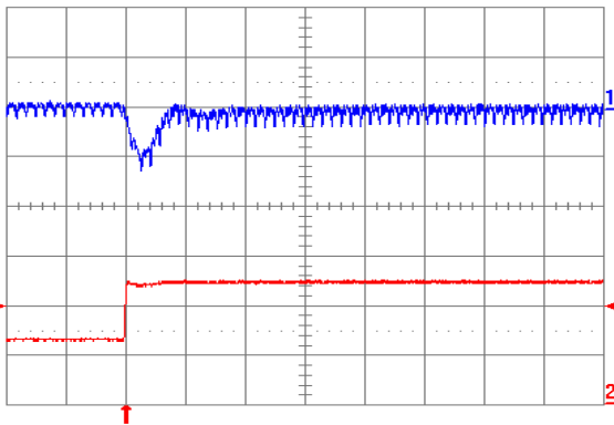
Fig. 1.8V.7: Output voltage response for V_{out} = 1.8V to a positive load current step change from 2.5A to 5A with a slew rate of 5A/\mu s at V_{in} = 12V . Top trace: output voltage (100mV/div); Bottom trace: load current (2A/div). C_o = 47\mu F ceramic. Time scale: 20 \mu s /div.
