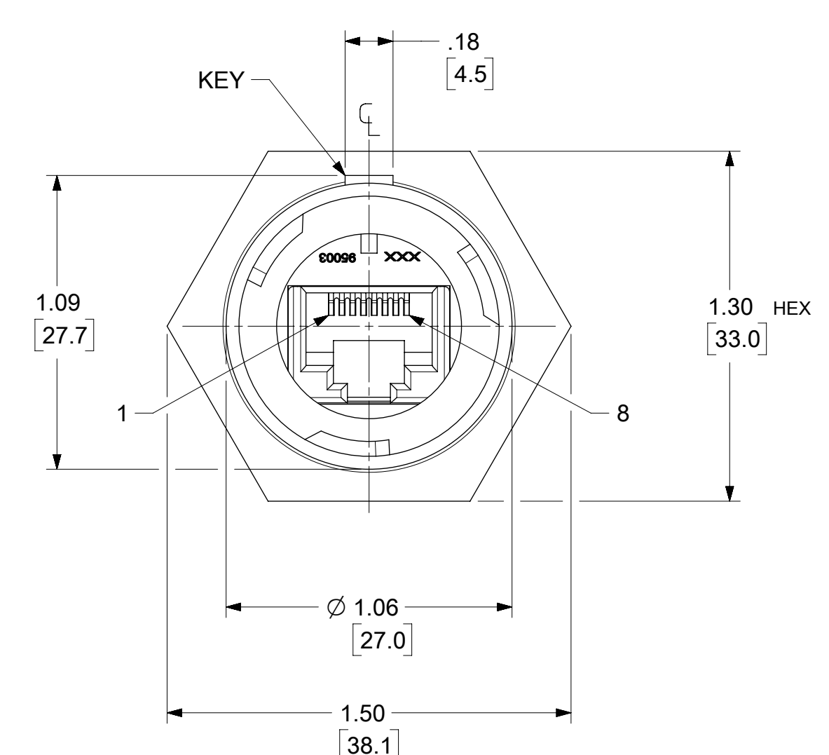
RJ45 FACE VIEW REF. TIA/EIA 568B
