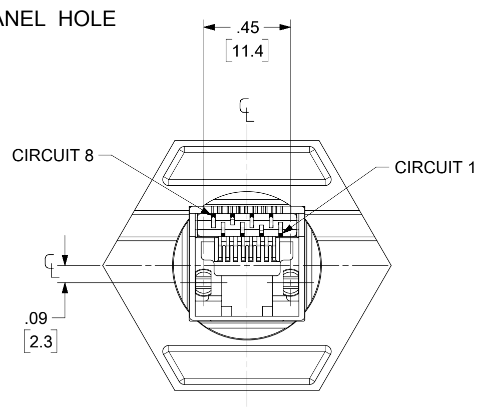
RJ45 BACK VIEW
