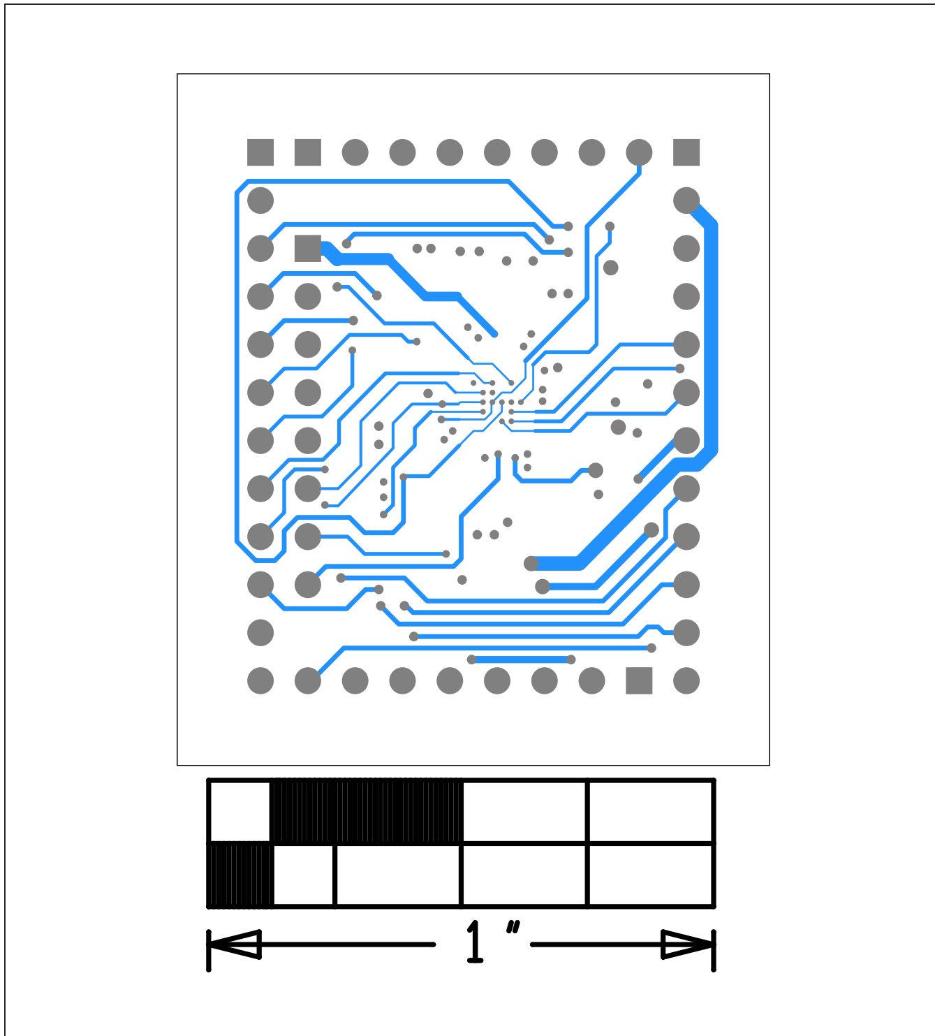
MAX20303 EV Kit—Bottom Copper
