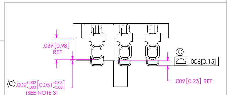
DETAIL 'F' SCALE 10:1
