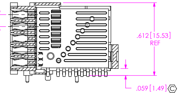
SECTION "D"-"D" SCALE 2 : 1
