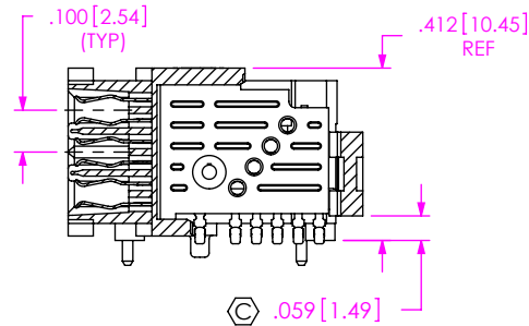
SECTION "B"-"B" SCALE 2 : 1
