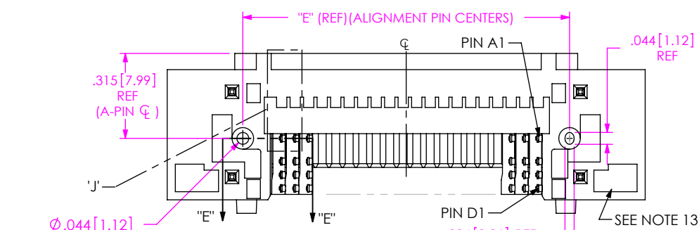
FIG 1 (SEAF-20-01-X-04-X-RA-GP) (SOME DETAIL OMITTED FOR CLARITY)
