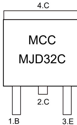
Device Marking
