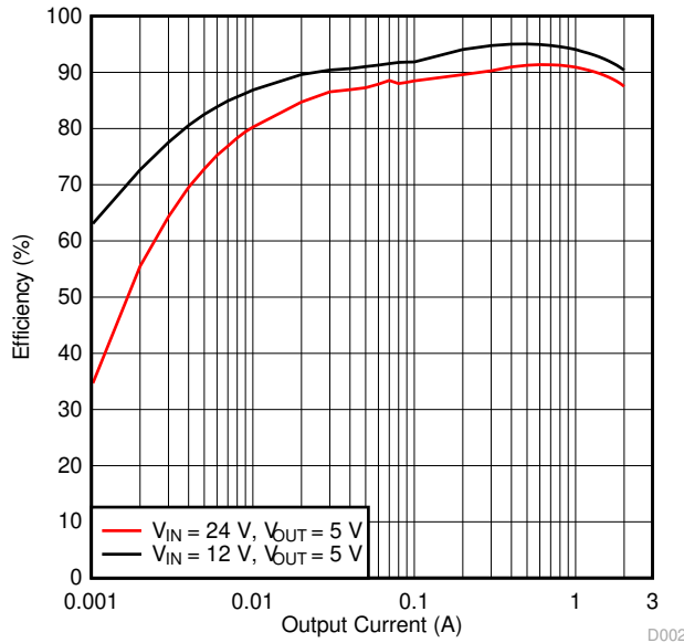
Figure 2-2. TPS54202HEVM-716 Low Current Efficiency
