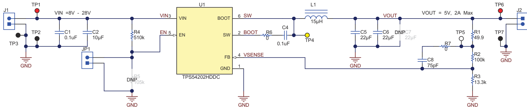
Figure 4-1. TPS54202HEVM-716 Schematic
