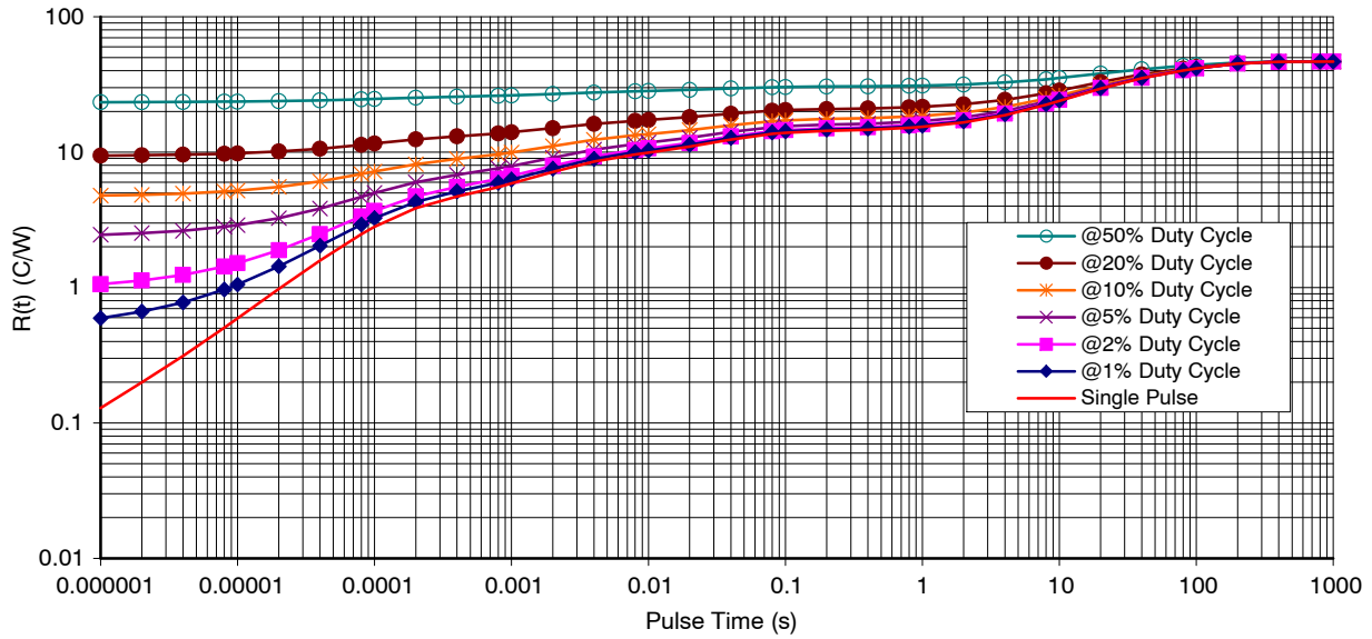
Figure 13. Thermal Characteristics
