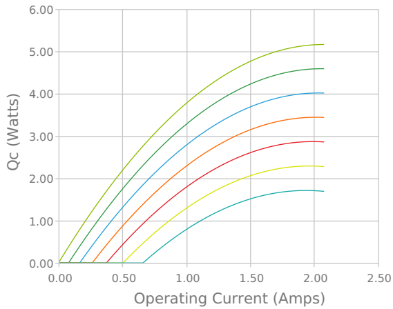
Heat Pumped at Cold Side T_{hot} = 85\text{ }^{\circ}\text{C}
