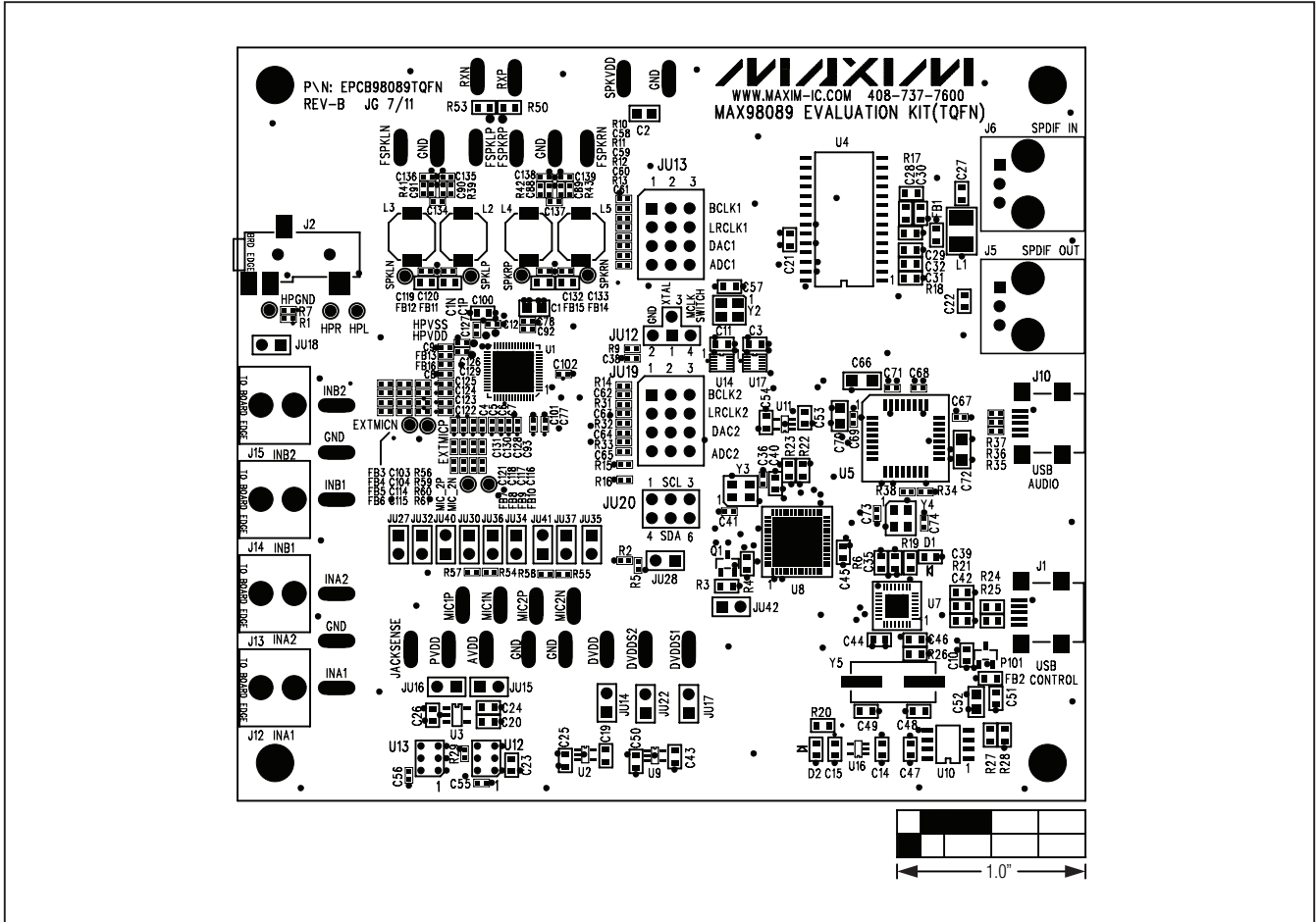
Figure 5. MAX98089 EV Kit Component Placement Guide—Component Side
