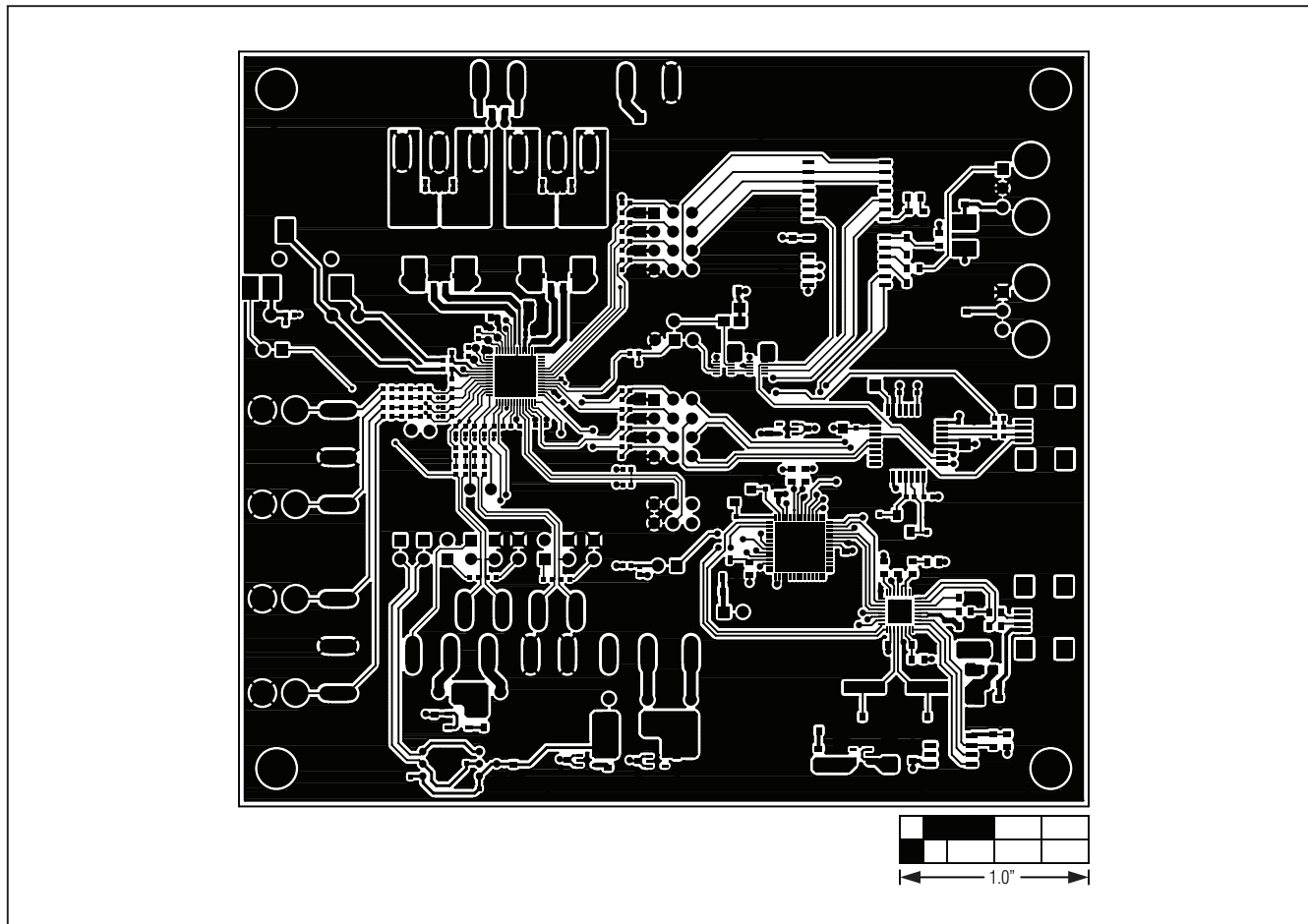
Figure 6. MAX98089 EV Kit PCB Layout—Component Side
