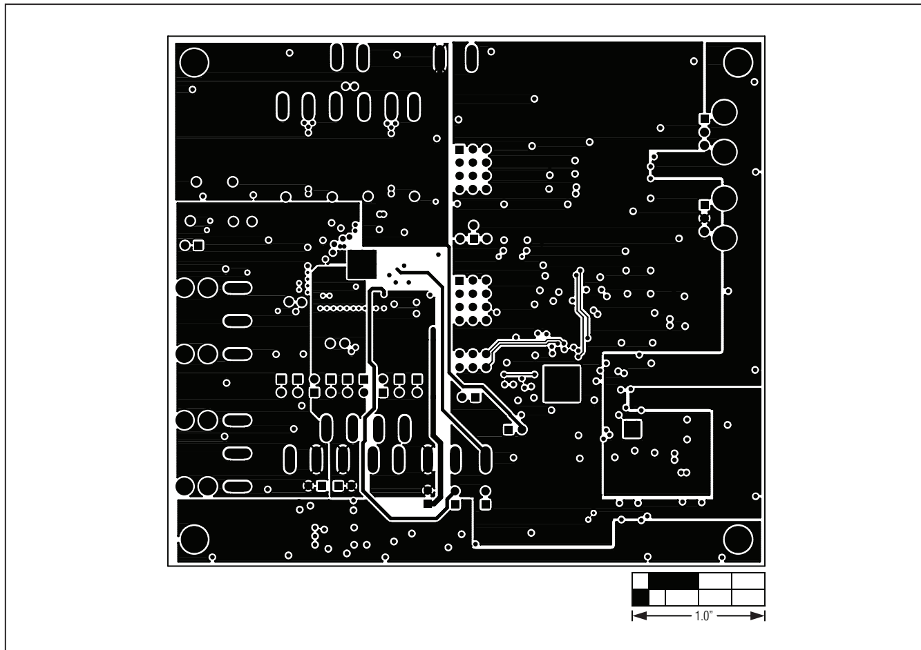
Figure 8. MAX98089 EV Kit PCB Layout—Power Layer 3
