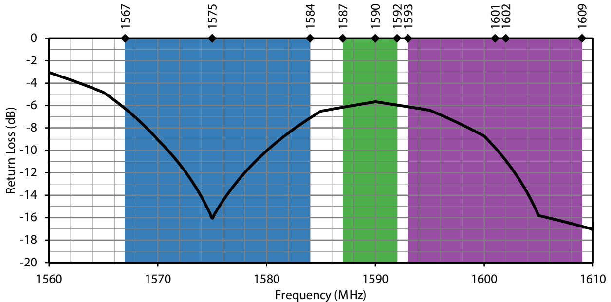
Figure 3. GNSSCP-TH18L1 Return Loss
