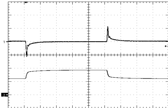
Figure 9. Load Transient Response (100mV/div), di/dt=0.1A/uS, 50% - 75% - 50% of full load, Cout=0 time scale: 200uS/div. Ch2 = 10A/div
