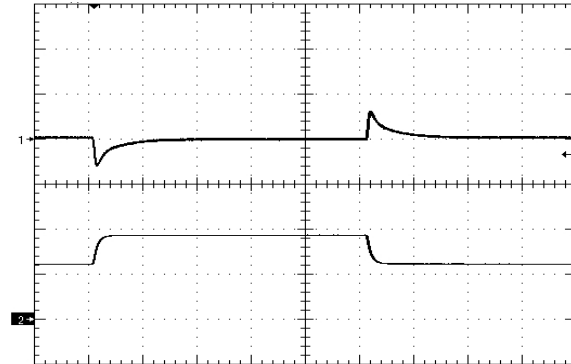
Figure 10. Load Transient Response (100mV/div), di/dt=0.5A/uS, 50% - 75% - 50% of full load +2200uF electrolytic, time scale: 200uS/div. Ch2 = 10A/div
