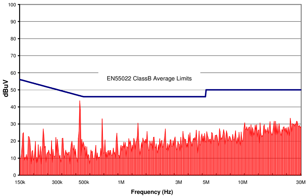
Figure 17. CPT25F48N Conducted Emissions using above specified input filter. Vin = 48V, Full Resistive Load
