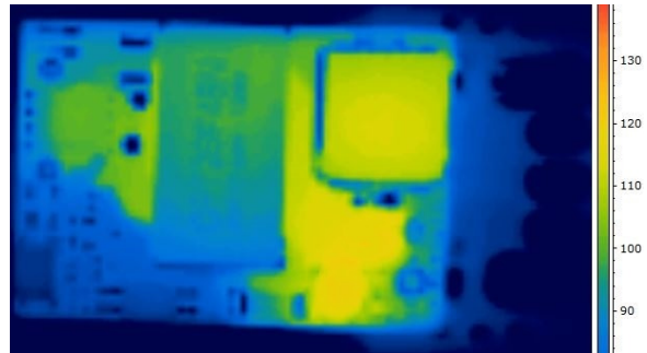
Figure 4. Thermal Image of CPT25F48 (25A output, 40C Ambient, 400lfm airflow, Vin = 48V, airflow from pin 3 to pin 1, T max = 122°C)
