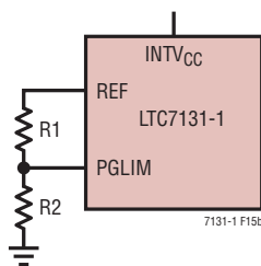
(b) PGOOD Window Set by R1/R2
