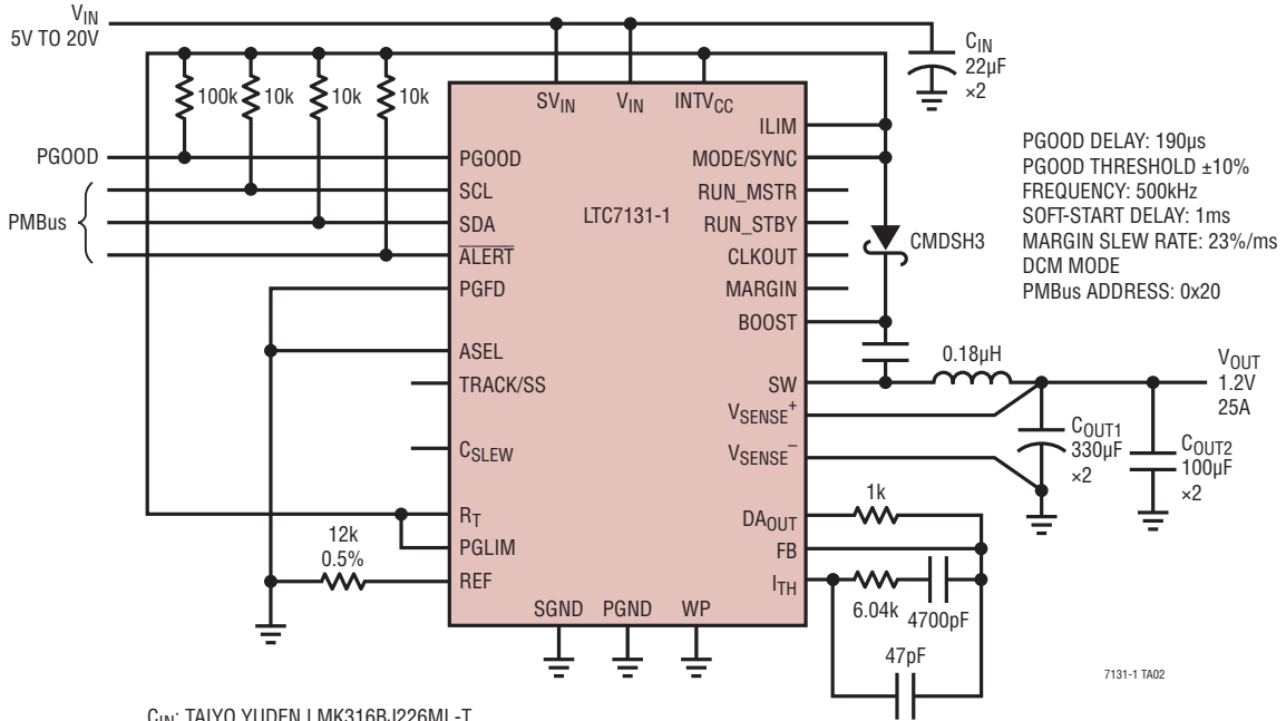
1.2V/25A 500kHz Buck Regulator with Minimum External Components
