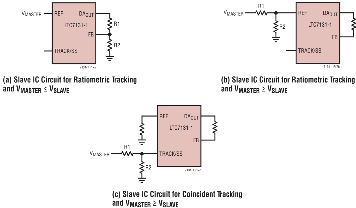
Figure 17. Slave IC Circuits
