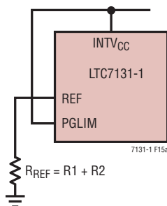
(a) PGOOD Window Set to \pm 10\% Default
