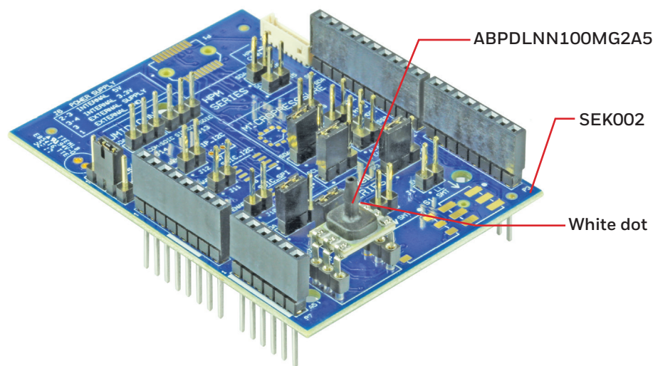
Figure 1. ABPDLNN100MG2A5 Mounted on the SEK002
