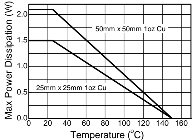
Derating Curve
