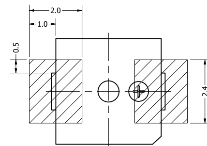
Land Pattern
