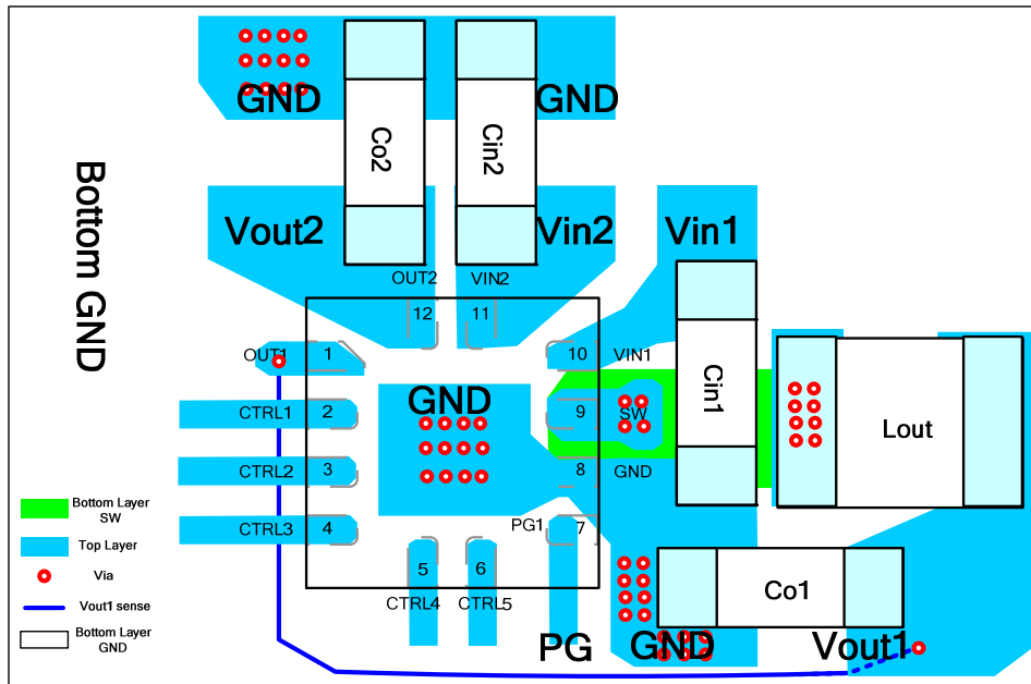
Figure 2: Recommended Layout
