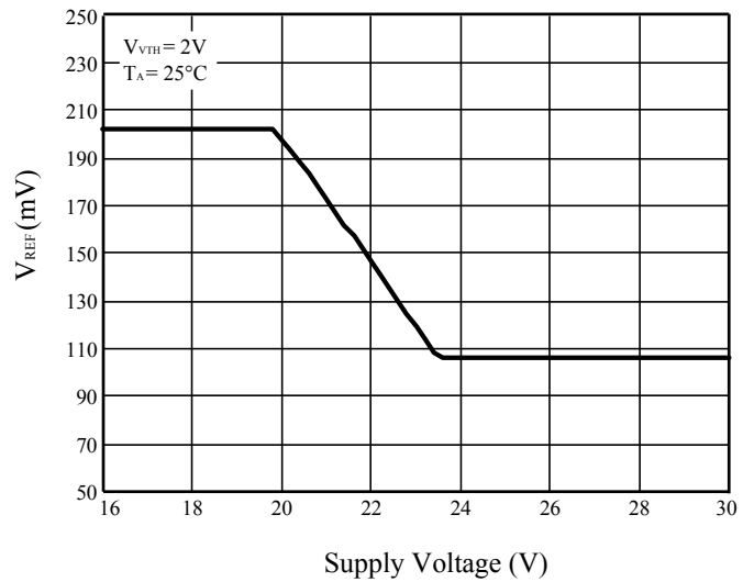
Figure 26 V_{REF} vs. Supply Voltage
