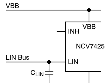
Figure 4. Slave Configuration
