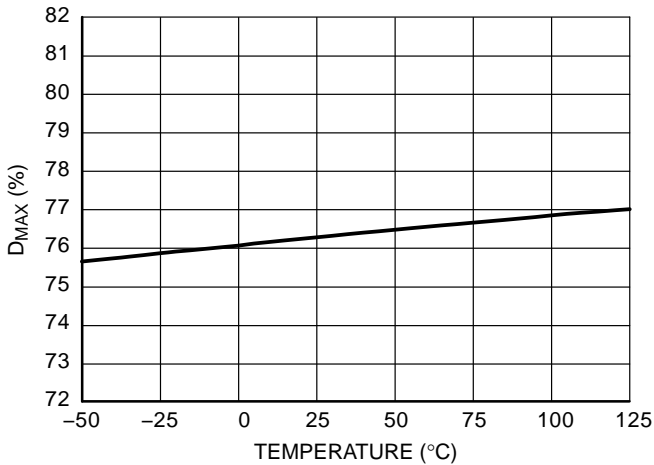
Figure 25. Maximum Duty Ratio D_{MAX}
