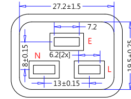
FM-319 (IEC 60320, C19, 20A 250V~) (Dimensions of Connector Face)
