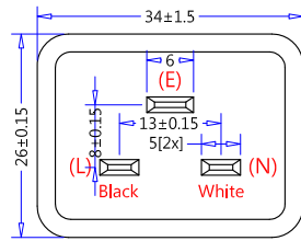
FM-320 (IEC 60320, C20, 20A 250V~) (Dimensions of Inlets Face)
