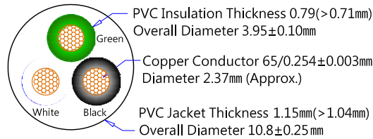
SJT 12AWGx3C 截面圖 (Wire Cross-Section)
