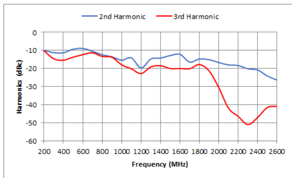
Harmonics (@ Psat)
