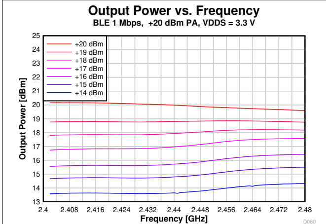
Figure 8-31. Output Power vs. Frequency (BLE 1 Mbps, 2.44 GHz, +20 dBm PA)
