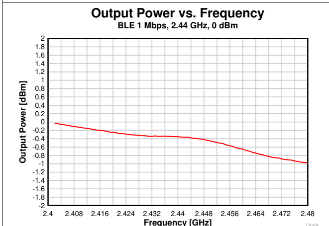
Figure 8-29. Output Power vs. Frequency (BLE 1 Mbps, 2.44 GHz)
