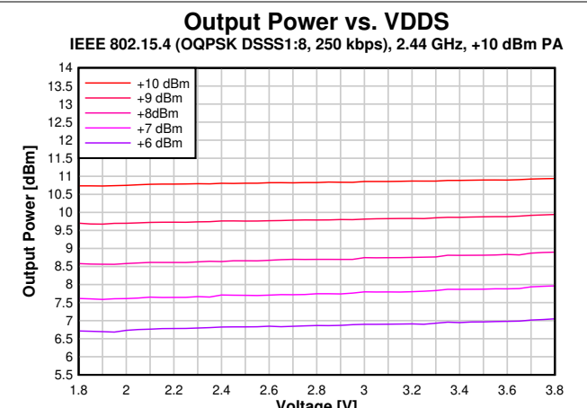
Figure 8-28. Output Power vs. Supply Voltage (VDD) (2.44 GHz, +10 dBm PA)
