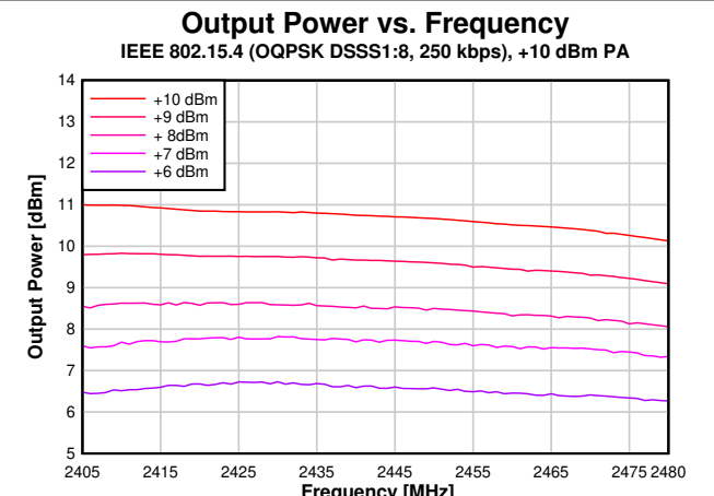
Figure 8-32. Output Power vs. Frequency (250 kbps, +10 dBm PA)
