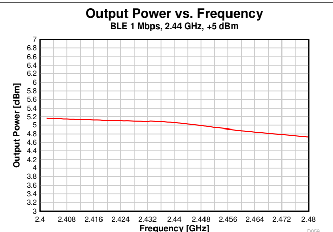
Figure 8-30. Output Power vs. Frequency (BLE 1 Mbps, 2.44 GHz, +5 dBm)
