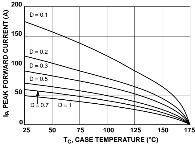
Figure 3. Current Derating
