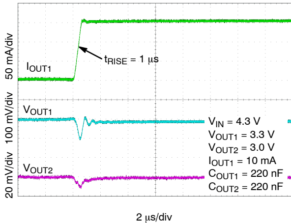
Figure 46. Load Transient Response – Rising Edge, I_{OUT} = 0.1 mA to 150 mA
