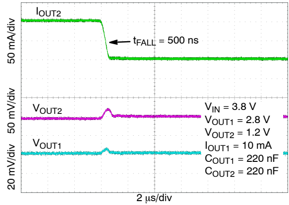
Figure 45. Load Transient Response – Falling Edge, I_{OUT} = 150 mA to 50 mA
