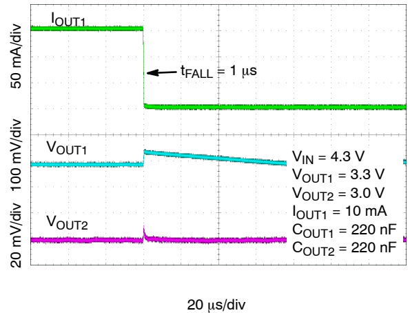
Figure 49. Load Transient Response – Falling Edge, I_{OUT} = 150 mA to 0.1 mA
