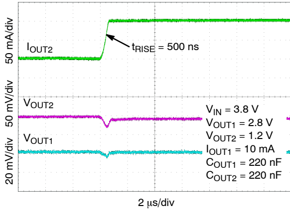
Figure 44. Load Transient Response – Rising Edge, I_{OUT} = 50 mA to 150 mA
