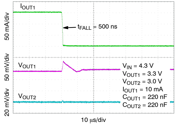
Figure 48. Load Transient Response – Falling Edge, I_{OUT} = 150 mA to 1 mA
