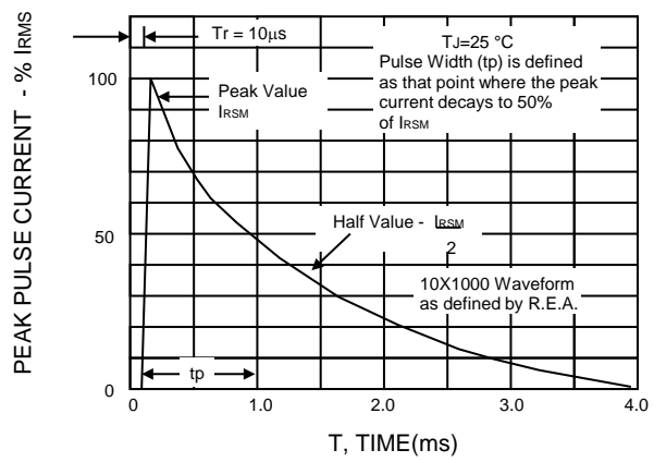
FIG.2 - PULSE WAVEFORM
