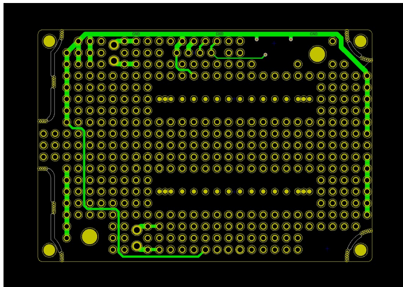
Pic.8. AMC PCB Back Copper traces
