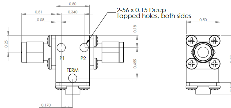
D3I3743Q-3 Dimensions
