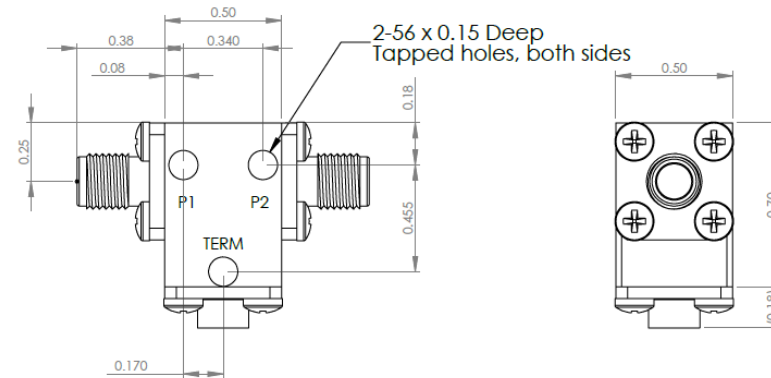
D3I3743Q Dimensions
