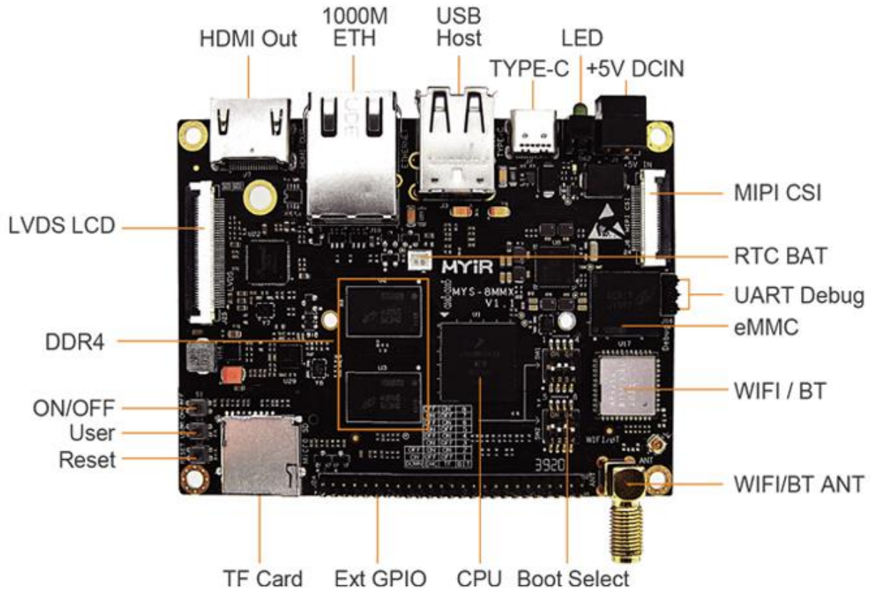
Figure 1-2 MYS-8MMX Top-View
