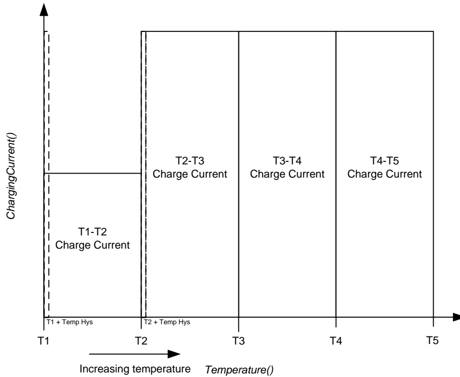
Figure 7-3. Temperature Hysteresis for Charging Current
