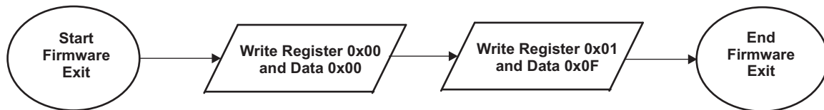
Figure B-4. Commands to Enter ROM Mode in HDQ
