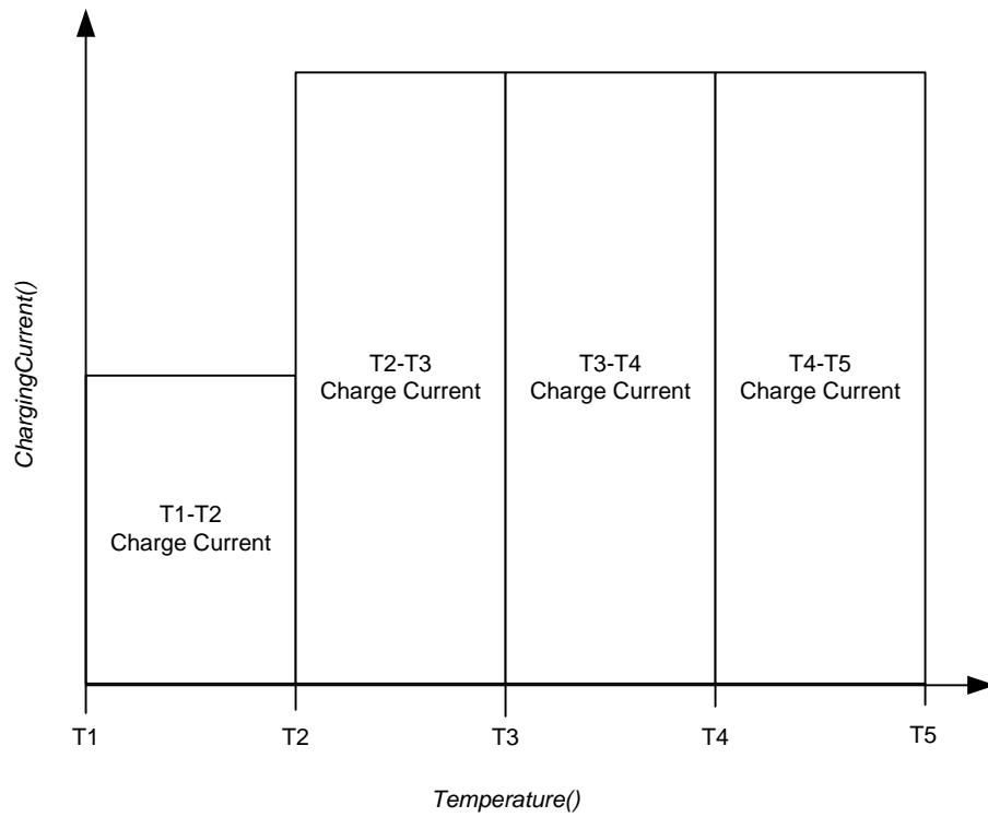
Figure 7-1. JEITA Charging Current Profile
