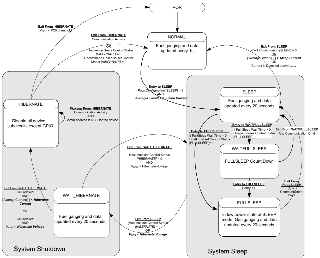
Figure 3-1. Power Mode Diagram—System Sleep
