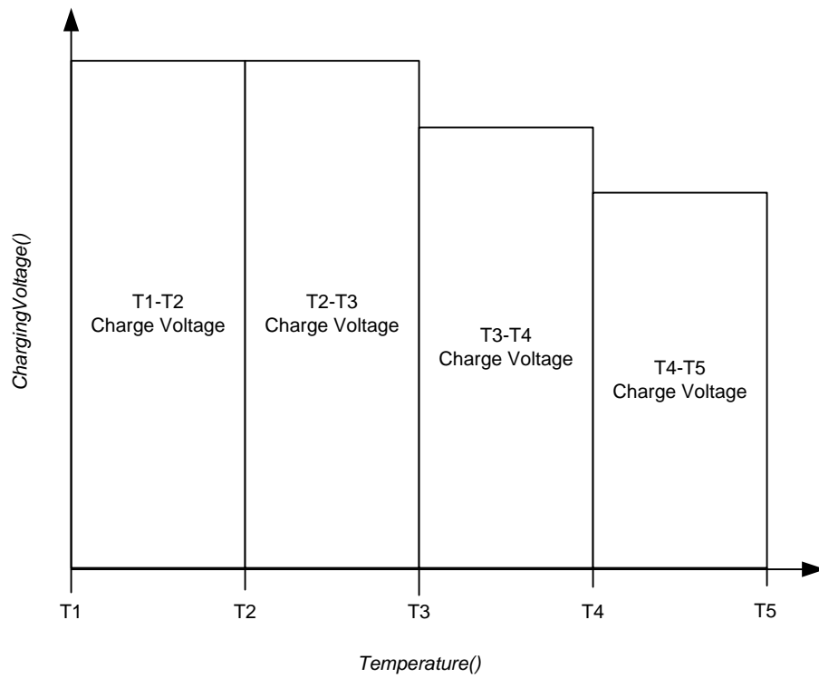
Figure 7-2. JEITA Charging Voltage Profile
