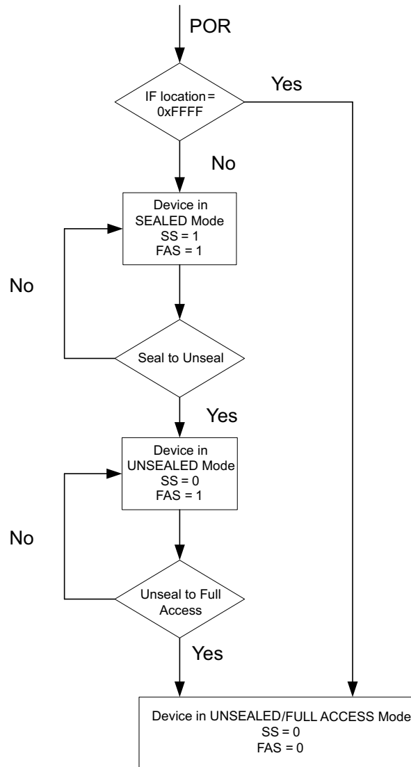
Figure 16-1. Gauge Mode State Diagram
