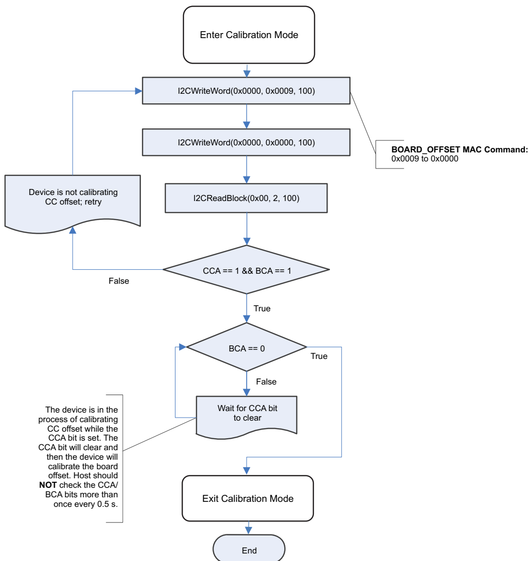
Figure A-2. Board Offset Flow
