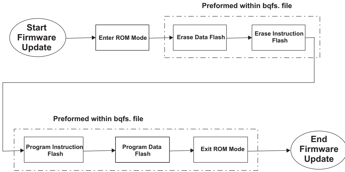
Figure B-2. Basic Firmware Programming Flow
