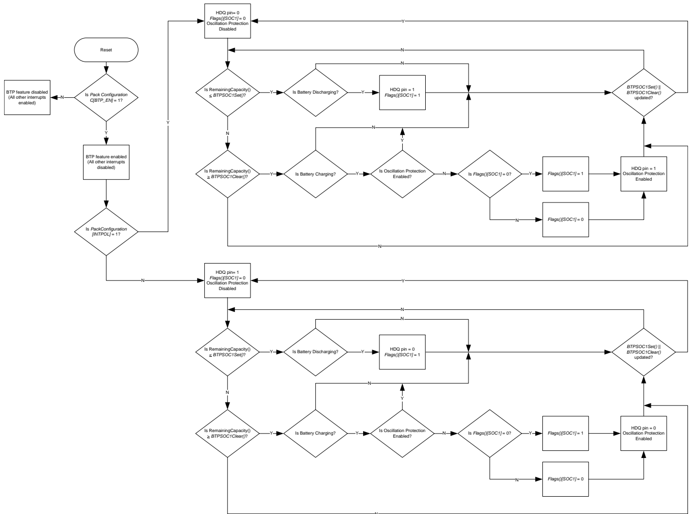
Figure 5-1. BTP Algorithm Flow
