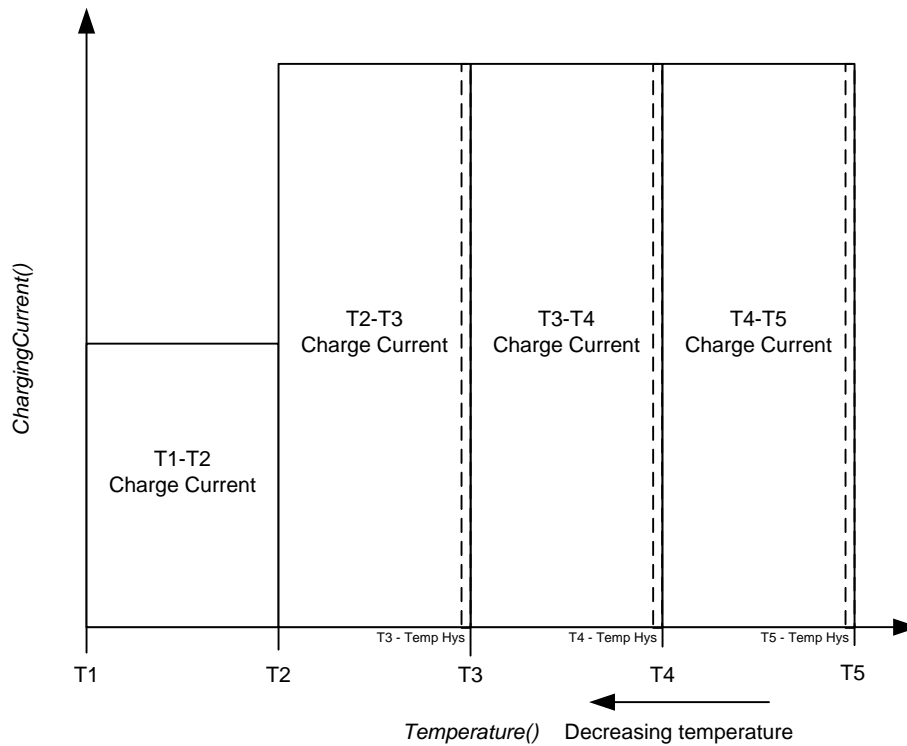
Figure 7-4. Temperature Hysteresis for Charging Voltage
