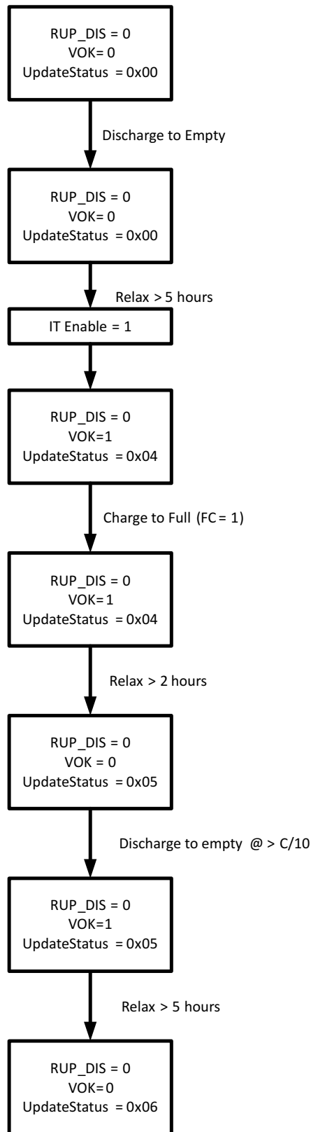
Figure C-2. Update Status Learning Cycle Diagram
