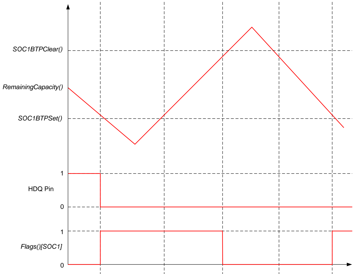
Figure 5-4. BTP Configuration with Separate Thresholds
