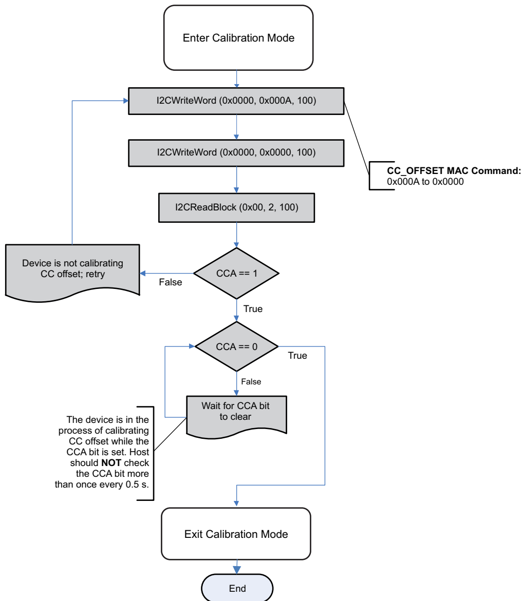
Figure A-1. CC Offset Flow
