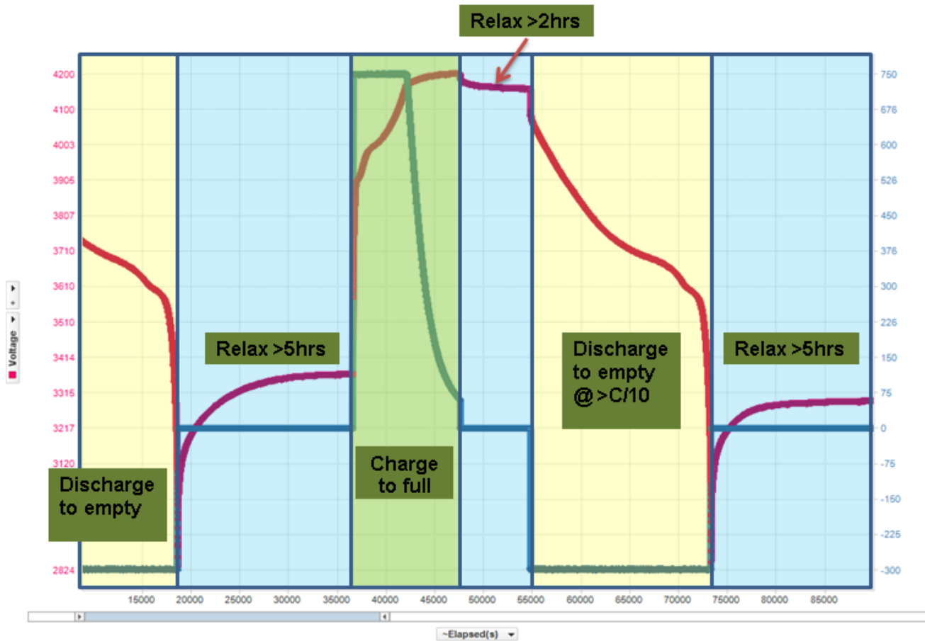
Figure C-1. Voltage/Current
