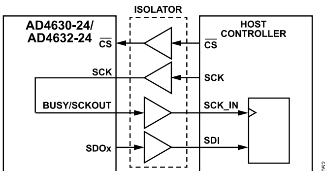
Figure 53. Echo Clock Mode Signal Path Diagram
