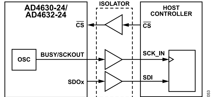
Figure 54. Host Clock Mode Signal Path Example
