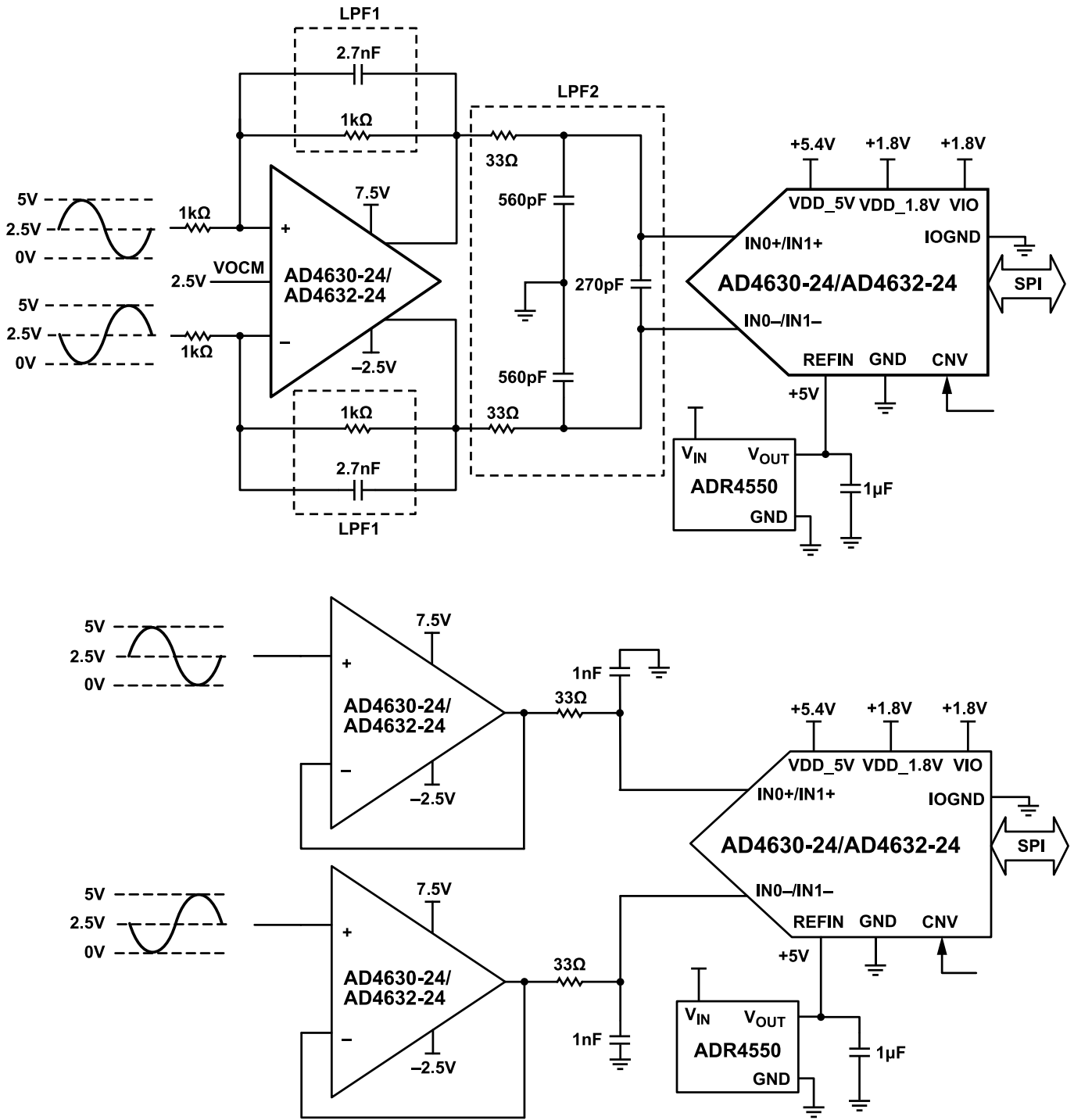
Figure 44. Typical Application Circuit Diagrams
