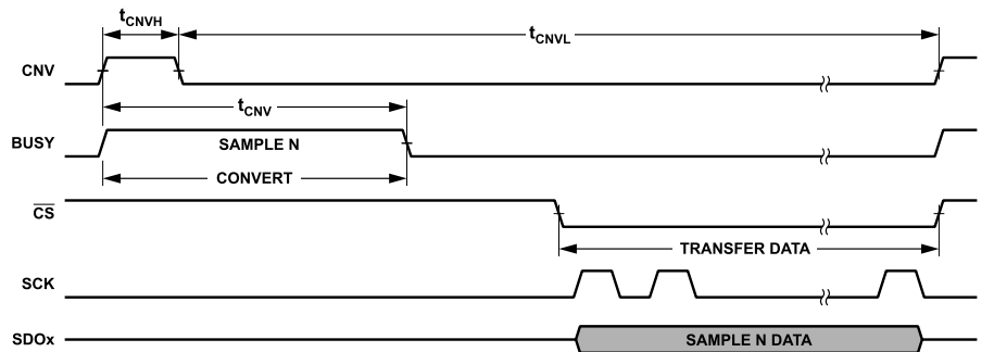
Figure 55. Basic Single Sample Conversion Cycle
