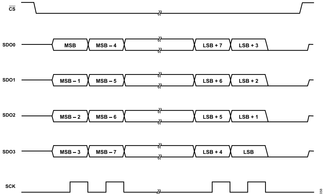
Figure 58. 4-Lane, SDR Timing Diagram
