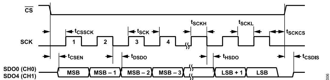
Figure 6. SPI Clcking Mode 1-Lane SDR Timing
