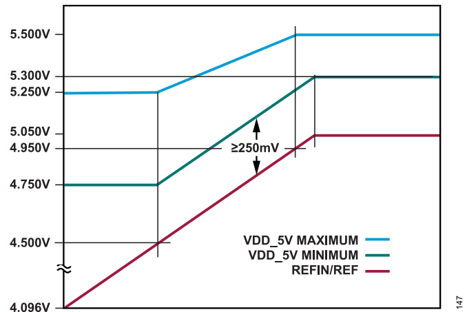
Figure 48. \text{VDD\_5V} Minimum and Maximum Values for \text{REFIN/REF}
