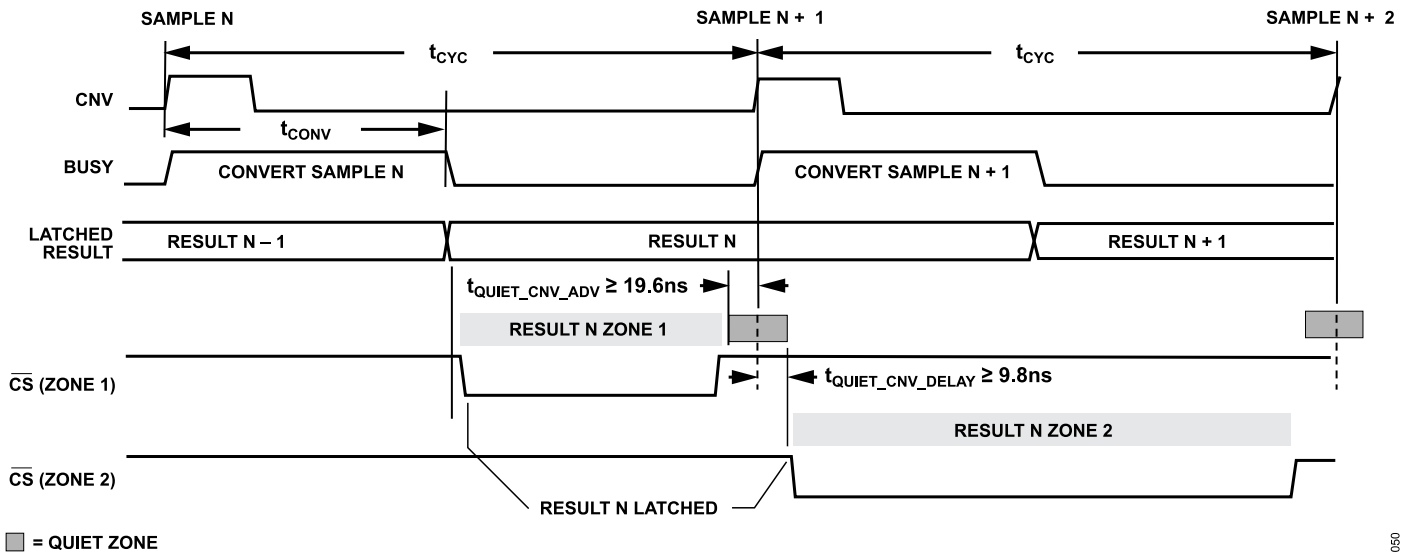
Figure 51. Example Timing for Data Transfer Zones
