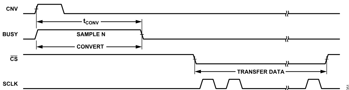
Figure 52. Typical Sample Cycle for SPI Clocking Mode
