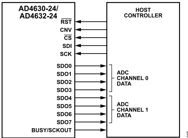
Figure 49. Multilane SPI
