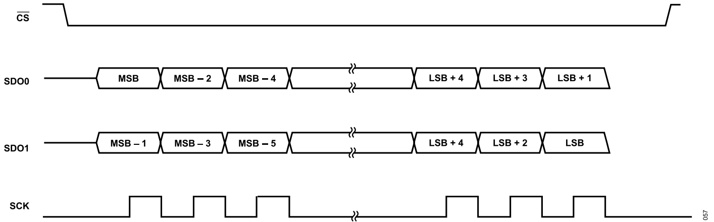
Figure 57. 2-Lane Mode, SDR Timing Diagram
