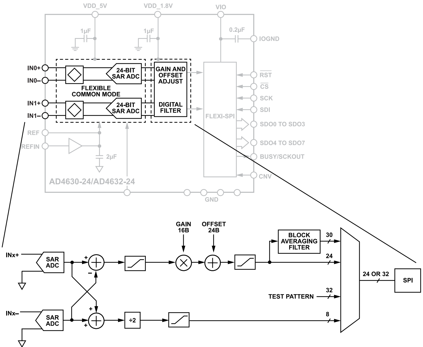
Figure 39. Functional Block Diagram and Channel Architecture
