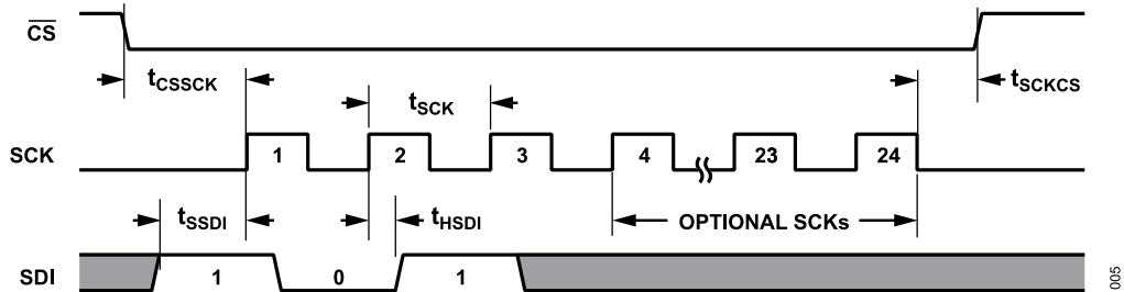
Figure 5. Register Configuration Mode Command Timing
