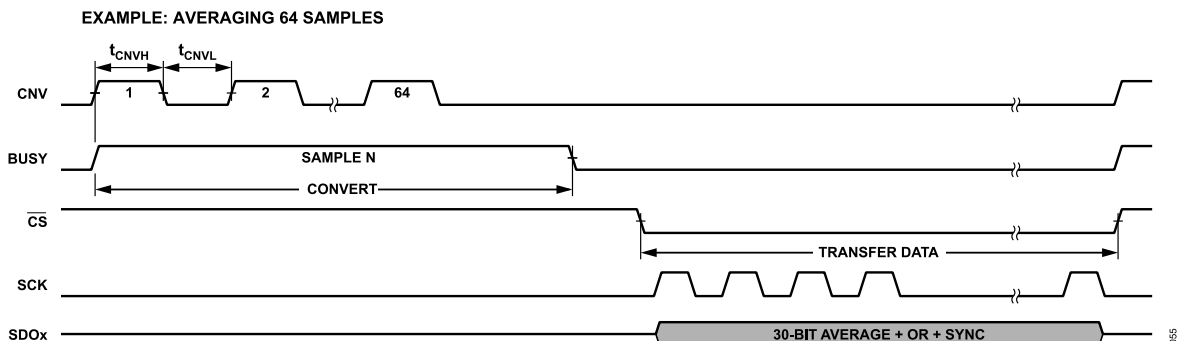
Figure 56. Example Conversion Cycle for Averaging Mode
