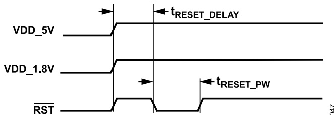
Figure 47. Power-On Reset (POR) Timing
