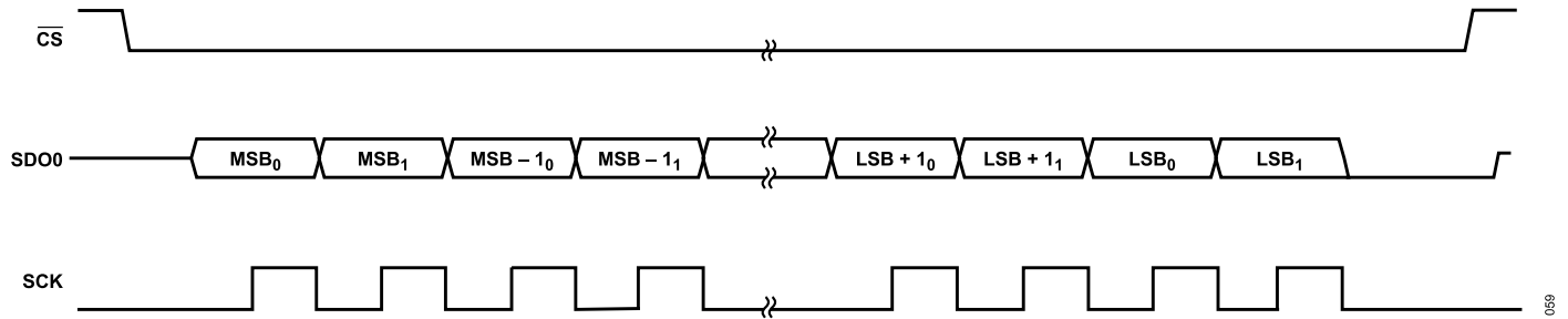
Figure 59. Interleaved Mode, SDR Timing Diagram
