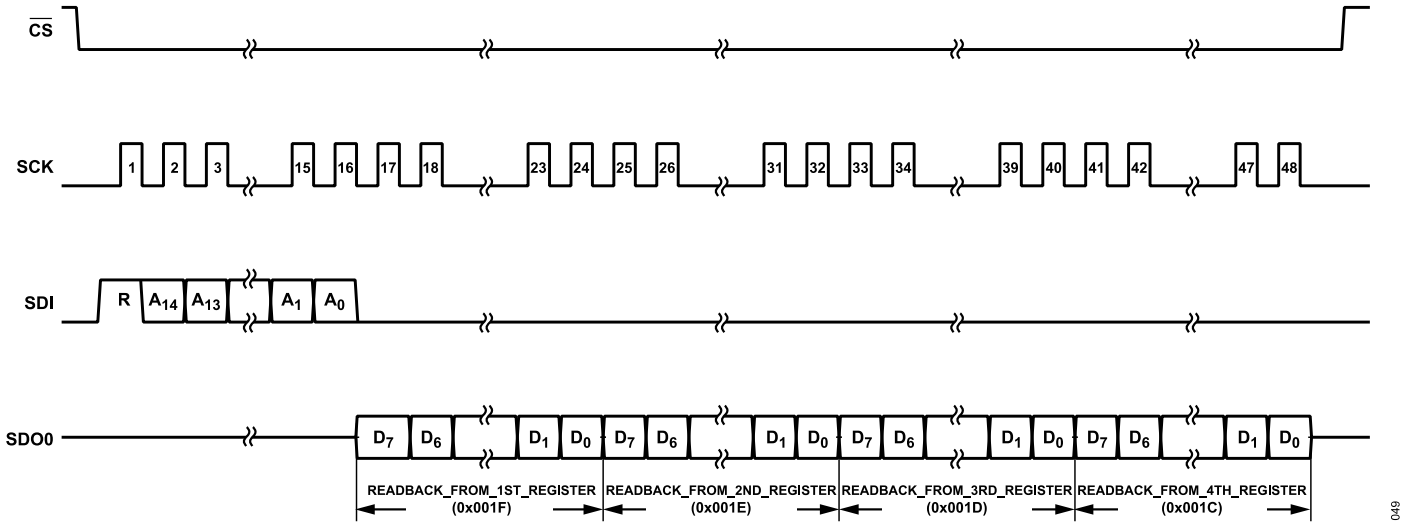
Figure 50. Stream Mode Bulk Register Read Back Operation
