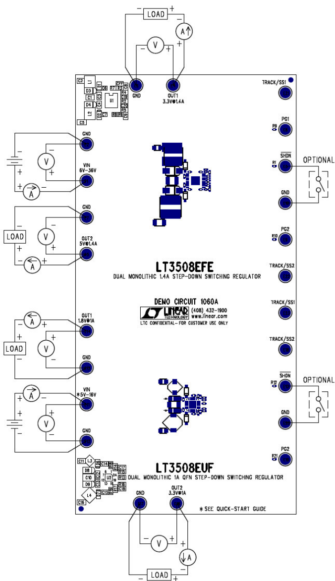
Figure 3. Proper Measurement Equipment Setup
