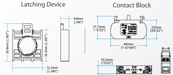
Non-Illuminated Operator (shown with Flush Cap)
