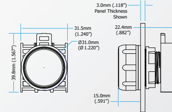
Illuminated Full Voltage and Multi-Voltage Dual Push Button Operators (shown with 1 Flush Cap and 1 Extended Cap)
